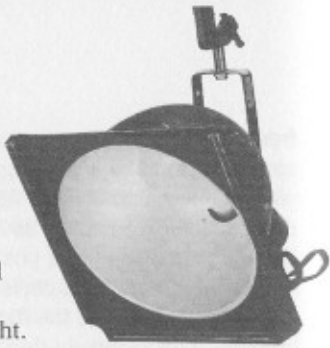
Scoop with rotatable square color-holder slot
