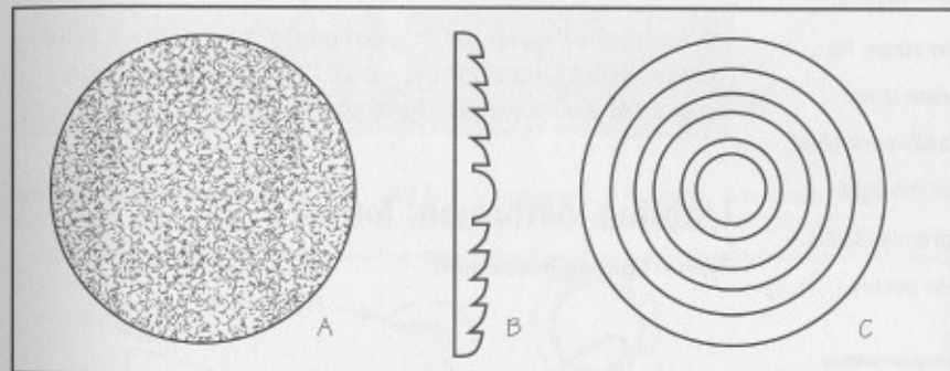
Fresnel lens: (A) back; (B) section; (C) front
