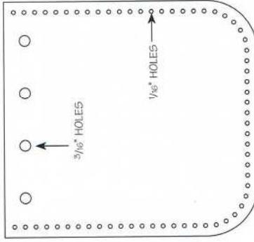
CUTTING PATTERN FOR LEATHER POUCH (REDUCED), FRONT AND BACK
