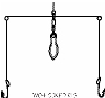
TWO-HOOKED RIG
