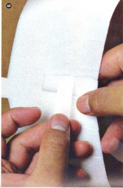
Step 6 —To attach the tail to the wing, slide slot 1 into slot 2. Making sure the tail is perpendicular to the wings, use two small pieces of tape (about 2 inches long) to secure the bottom of the tail to the bottom of the wing.
