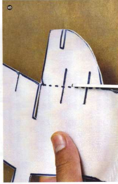
Step 5 —Cut along the dotted line to separate the tail from the wings. For ease, make all of your cuts from the outside of the plate toward the center of the plate. Don't try to turn the scissors to make sharp corners. Cut the two slots only as wide as the thickness of the foam plate; otherwise the pieces will not fit together snugly.
