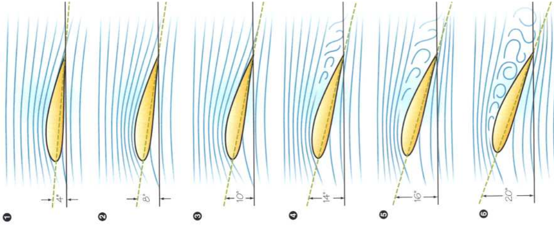
How airfoils work
