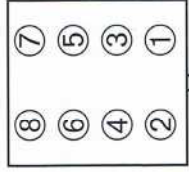
V-8 OR BOXER: 1-8-4-3-6-5-7-2
